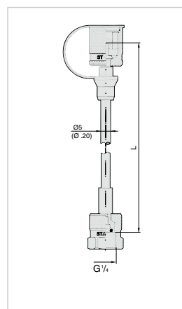
Gauge Adaptor
