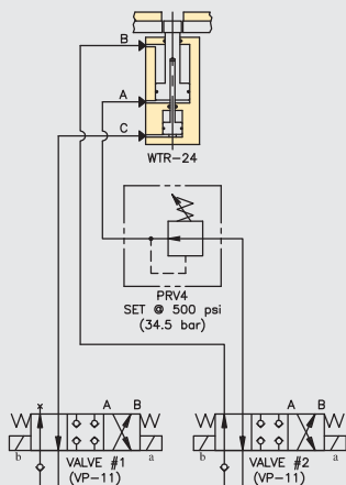
Clamp
