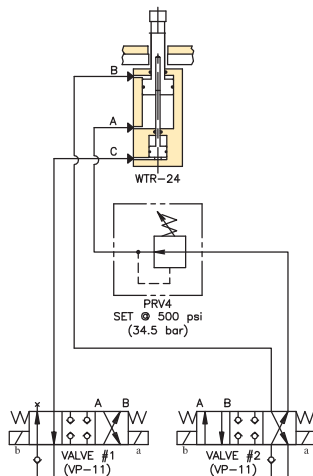
Clamp Hold
