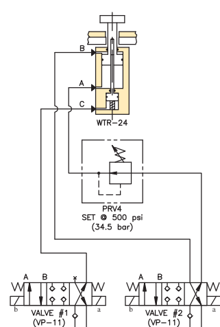
Unclamp
