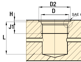
Installation dimensions
