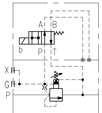
Pressure Relief, normally high pressure, energize to unload
