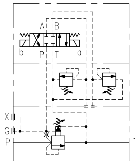
Pressure Relief, 3 pressure, normally highest pressure, energize A solenoid for pressure setting A energize B solenoid for pressure setting B
